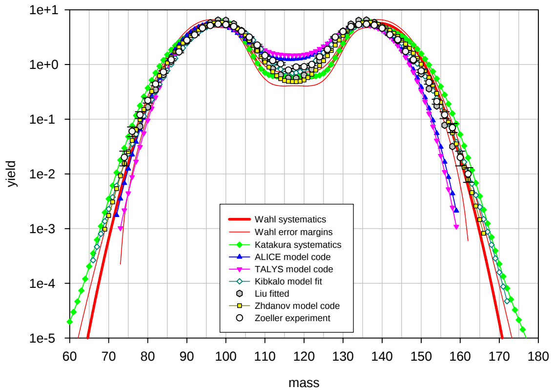
Benchmark A: ^{238}\text{U} around 13 MeV, post neutron emission fission yields
